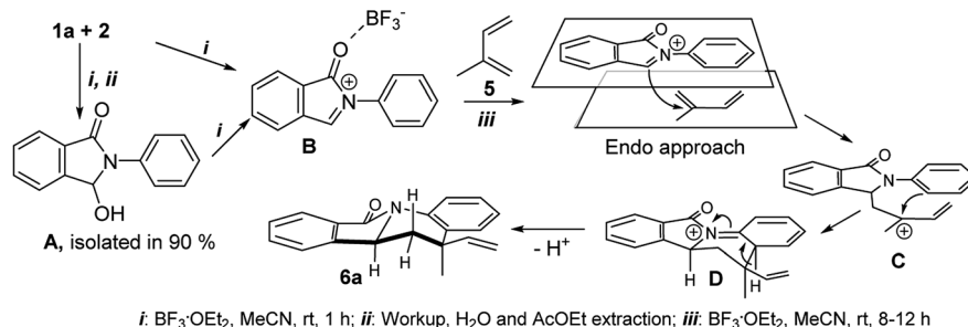
Scheme 2 Mechanistic proposal of the isoindolo[2,1-a]quinolin-11(5H)-one skeleton formation.
