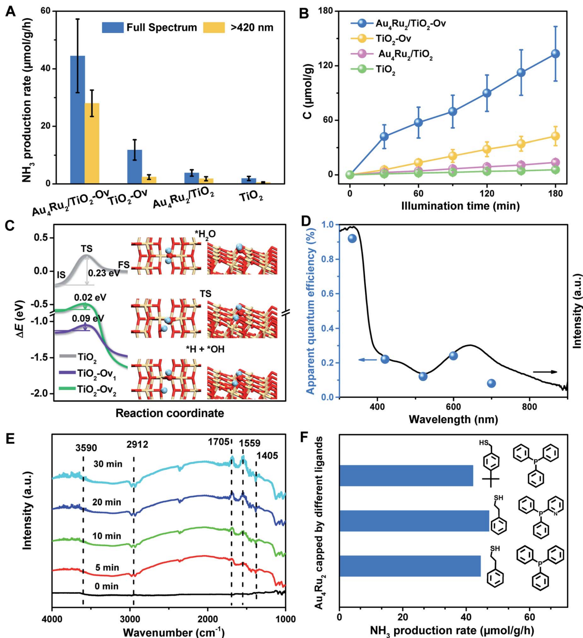
Fig. 3 (A) The photocatalytic performances of the \text{Au}_4\text{Ru}_2/\text{TiO}_2 -Ov, \text{Au}_4\text{Ru}_2/\text{TiO}_2 , \text{TiO}_2 -Ov and \text{TiO}_2 catalysts for \text{N}_2 reduction. (B) Time-dependent photocatalytic ammonia production over the \text{Au}_4\text{Ru}_2/\text{TiO}_2 -Ov, \text{Au}_4\text{Ru}_2/\text{TiO}_2 , \text{TiO}_2 -Ov and \text{TiO}_2 catalysts. (C) Reaction energy diagrams of water dissociation on the anatase \text{TiO}_2(101) surface without defect ( \text{TiO}_2 ) and with an oxygen vacancy per supercell on surface ( \text{TiO}_2 -Ov 1 ) and subsurface ( \text{TiO}_2 -Ov 2 ), respectively. \Delta E is relative to the energy of each substrate plus a free water molecule. Insets are the structures of water adsorption (top) and dissociation into ^*\text{H} and ^*\text{OH} species adsorbed on \text{TiO}_2 -Ov 1 (bottom), and the transition state (middle). The H, O and Ti are shown in cyan, red and yellow. (D) UV-DRS and quantum efficiency of \text{Au}_4\text{Ru}_2/\text{TiO}_2 -Ov for \text{NH}_4^+ evolution by photocatalytic \text{N}_2 reduction under monochromatic light of different wavelengths. (E) In situ FTIR spectra of the photocatalytic \text{N}_2 reduction over \text{Au}_4\text{Ru}_2/\text{TiO}_2 -Ov during full spectrum illumination in the presence of \text{N}_2 and water. (F) Performances of the \text{Au}_4\text{Ru}_2 clusters protected by different ligands for photocatalytic \text{N}_2 reduction.
