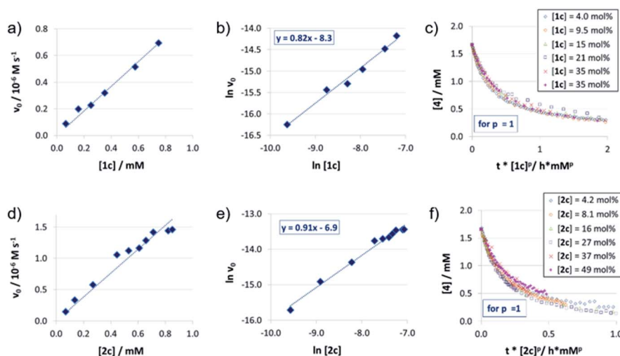
Fig. 2 Catalyst order determination for catalysts 1c (a, b, c) and 2c (d, e, f): initial rates (all at 1.66 mM quinoline 4 and 3.93 mM Hantzsch-ester 7 ) (a, d), \ln v_0 / \ln [\text{catalyst}] plots ( v_0 in \text{M}^{-1} \text{s}^{-1} , catalyst concentrations in M) (b, d) and VTNA-plots (selected catalyst concentrations only) (c, f).
