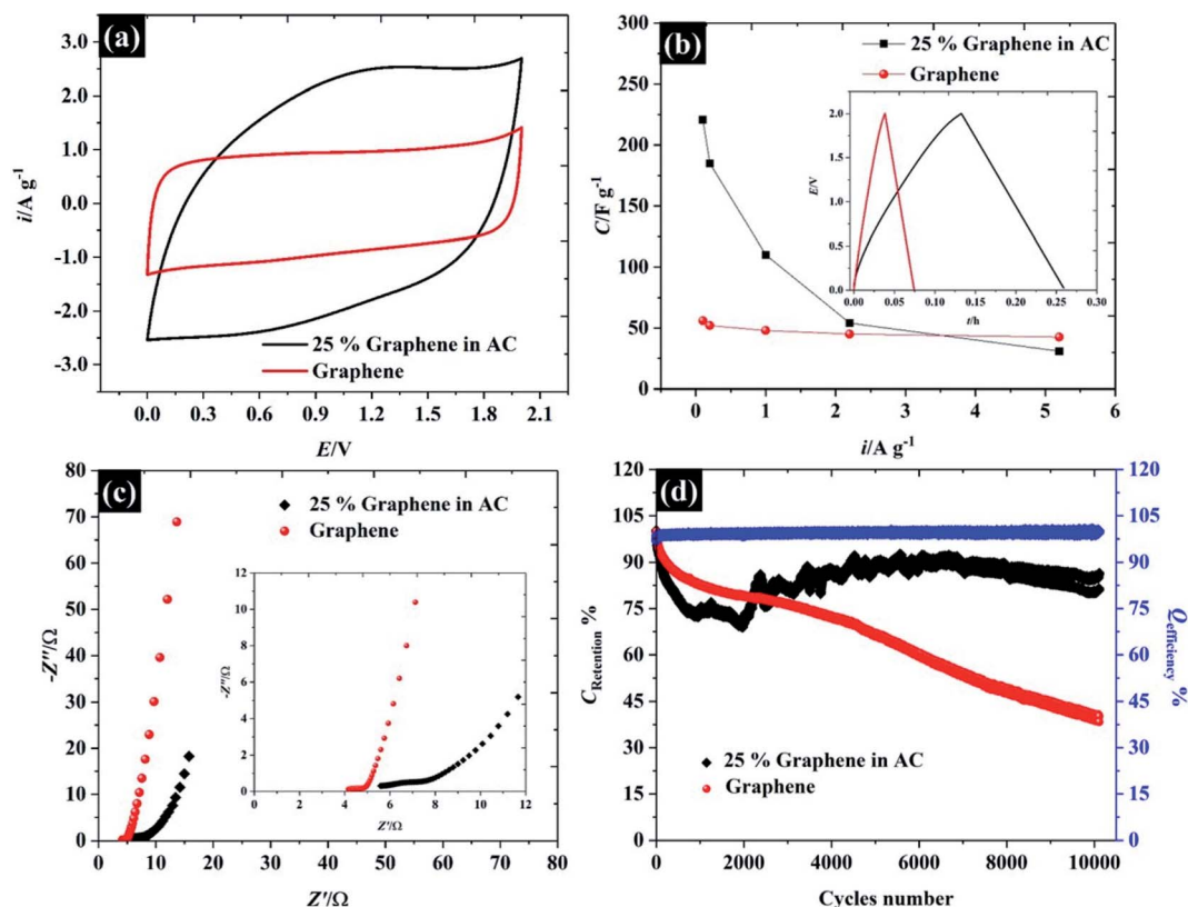
Fig. 9 Performance of supercapacitor devices using 17 M KF electrolyte. (a) CV at 75\ mV\ s^{-1} , (b) capacitance and charge/discharge profile at 2.2\ A\ g^{-1} , (c) Nyquist plot, and (d) cyclic stability at 1.0\ A\ g^{-1} over 10 000 cycles.
