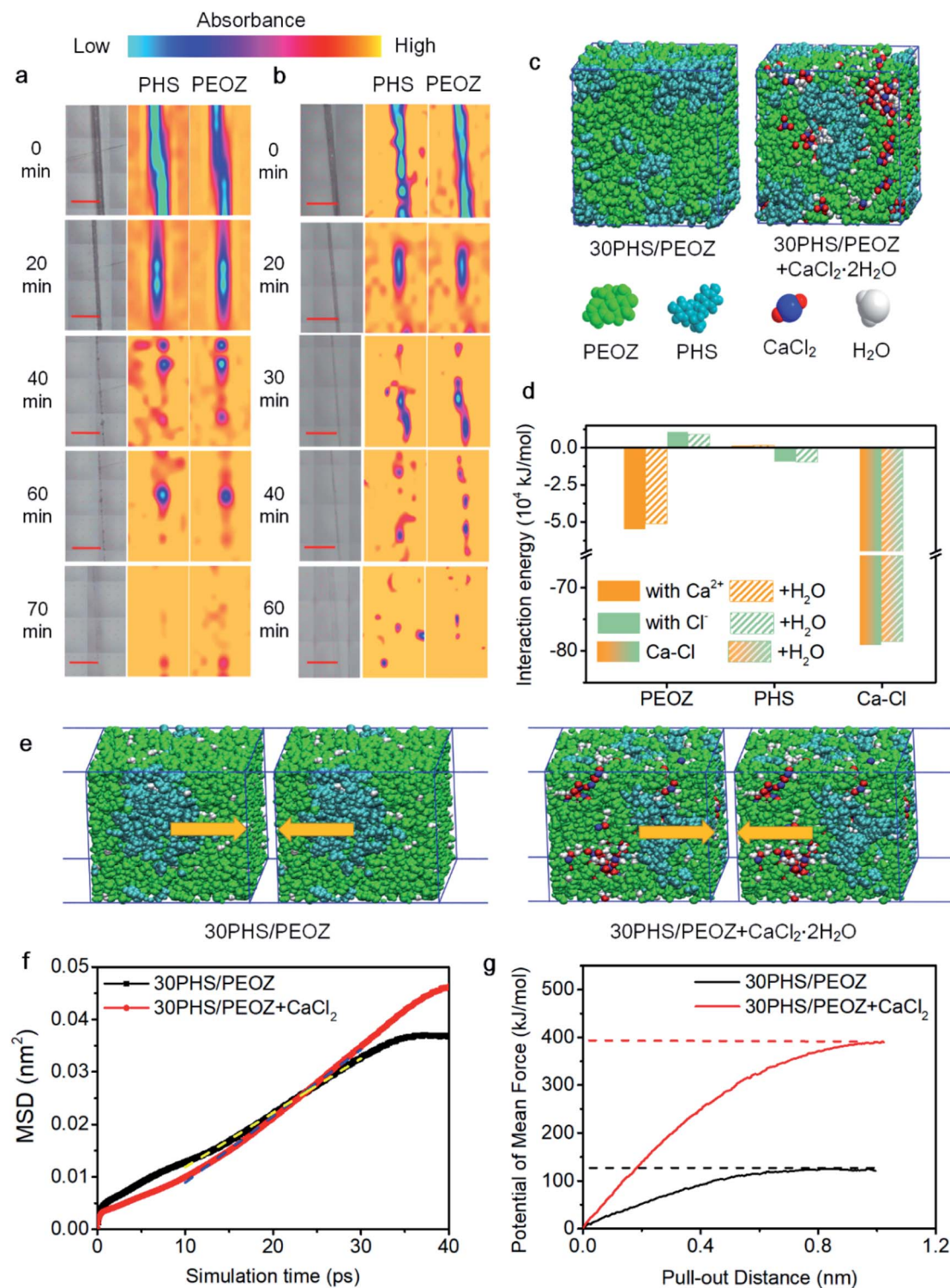
Fig. 3 Spectral mapping and the simulations of the self-healing process of 30PHS/PEOZ with \text{CaCl}_2 . The self-healing monitoring by micro-FTIR mapping analysis on the surface of (a) 30PHS/PEOZ and (b) 30PHS/PEOZ + \text{CaCl}_2 . The optical images display the scratched area of the films. The false-color mapping images, of which the peak at 1509\text{ cm}^{-1} refers to PHS, and the peak at 1624\text{ cm}^{-1} is assigned to PEOZ, indicate the distribution of PHS and PEOZ respectively during the self-healing process (scale bars: 100\text{ }\mu\text{m} ). (c) The computational cells of the 30PHS/PEOZ and 30PHS/PEOZ + \text{CaCl}_2 . (d) The interaction energy of PEOZ and PHS with \text{Ca}^{2+} and \text{Cl}^- , and the interaction energy between \text{Ca}^{2+} and \text{Cl}^- , respectively, “+ \text{H}_2\text{O} ” means wet condition. (e) The equilibrated configuration for the wet environment self-healing simulation. (f) Mean square displacement vs. simulation time of 30PHS/PEOZ and 30PHS/PEOZ + \text{CaCl}_2 . (g) The curves of the potential of mean force against the pull-out distance after self-healing.
