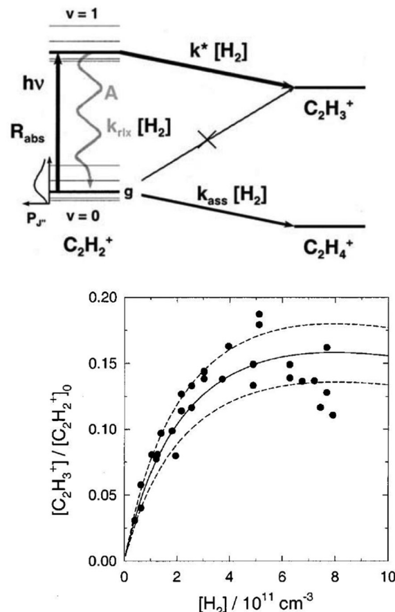
Fig. 3 (top) Level scheme for the LIR-process of \text{C}_2\text{H}_2^+ showing all radiative and collisional rates. (bottom) LIR-signal for the \text{P}(9) transition as a function of the \text{H}_2 number density, including three different solutions of the rate equation system. 38 Figures reprinted from ref. 38 with permission of AIP Publishing.
