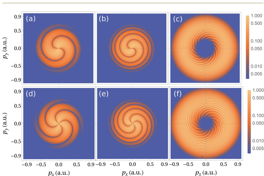
Fig. 4 Interference vortices from twisted electrons. Panels (a) and (b) show interference between photoelectrons with an OAM of \pm 1 , panels (d) and (e) show interference between photoelectrons with an OAM of \pm 2 , the left column uses a delay of 4 cycles, the middle column uses a delay of 1 cycle. The distributions are chosen to be Gaussian in momentum coordinates p_x and p_y . The right column shows the interference of the OAM distributions of the SFA [top] and RMT [bottom]. Gaussian distributions of twisted electron states are taken to reflect the OAM distributions shown in Fig. 3. Each panel is normalized with respect to its peak value and plotted on a logarithmic scale.
