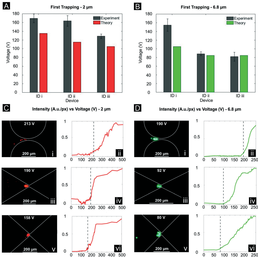
Fig. 5 Trapping voltages for different device and particle combinations. (A) First trapping voltage for the 2.0 \mu\text{m} particle. The bars in gray color show the first trapping voltage observed experimentally, the bars in red color show the first trapping voltages computed using eqn (6) (C i, iii, v) Total trapping voltage for device ID i, ID ii, and ID iii respectively (C ii, iv, vi) fluorescence intensity plotted as the applied voltage is increased until total trapping is achieved (B and D) in analogy to (A and C) figures are displayed in green for the 6.8 \mu\text{m} particle.
