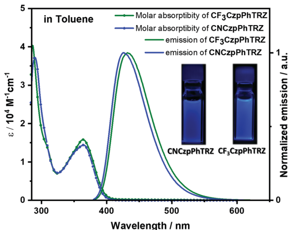
Fig. 3 Molar absorptivity and photoluminescence spectra of \text{CF}_3\text{CzpPhTRZ} and \text{CNCzpPhTRZ} in toluene at 298 K ( \lambda_{\text{exc}} = 360 nm). Inset: photos of photoexcited solutions in toluene.
