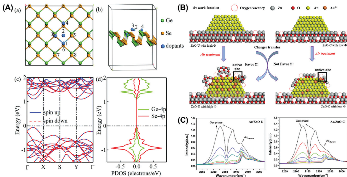
Fig. 14 Mechanism of dopant sites and creation of active sites for the introduction of noble metals. (A) Crystal lattice structure of noble metal-doped GeSe. (a) and (b) Location of doped metals with different perspectives. (c) Band structure and (d) partial density of states (PDOS) of monolayer GeSe. (B) Creation of active sites after Au doping with oxygen vacancy. (C) In situ FTIR spectra of CO adsorption for the study of adsorption sites and valence states of Au catalyst. (A) Reprinted from ref. 158. (B) and (C) reprinted from ref. 160.
