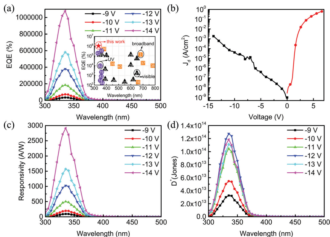
Fig. 2 (a) EQE, (b) J_{\text{d}} - V , (c) R , and (d) D^* characteristics of the fabricated UV PM-type OPDs under different applied voltages. The device structure is ITO/TAPC: C_{60} (50:1, 80 nm)/Al(100 nm). Inset of (a): summary of the peak EQEs of our prepared devices and the reported organic or organic/inorganic photodetectors.
