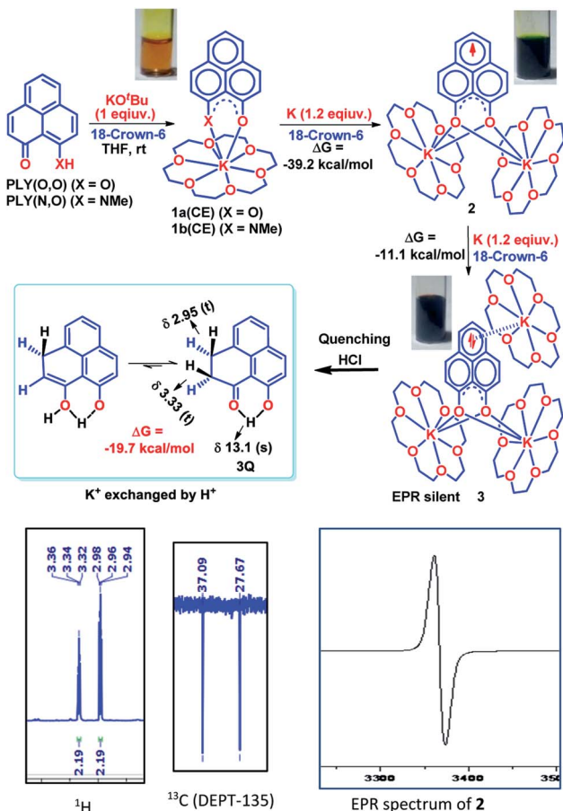
Scheme 1 Preparation of the PLY–K complexes (1a(CE) and 1b(CE), 12\pi\text{e}^- species) and consecutive one electron reduction by K to generate mono-reduced 13\pi\text{e}^- species (2) and doubly reduced 14\pi\text{e}^- species (3), respectively; quenching the 14\pi\text{e}^- species by replacing all \text{K}^+ ions with \text{H}^+ ions through HCl treatment; (insets: EPR spectrum of 2 and selected part of ^1\text{H} and ^{13}\text{C} (DEPT-135) NMR spectra of 3Q).
