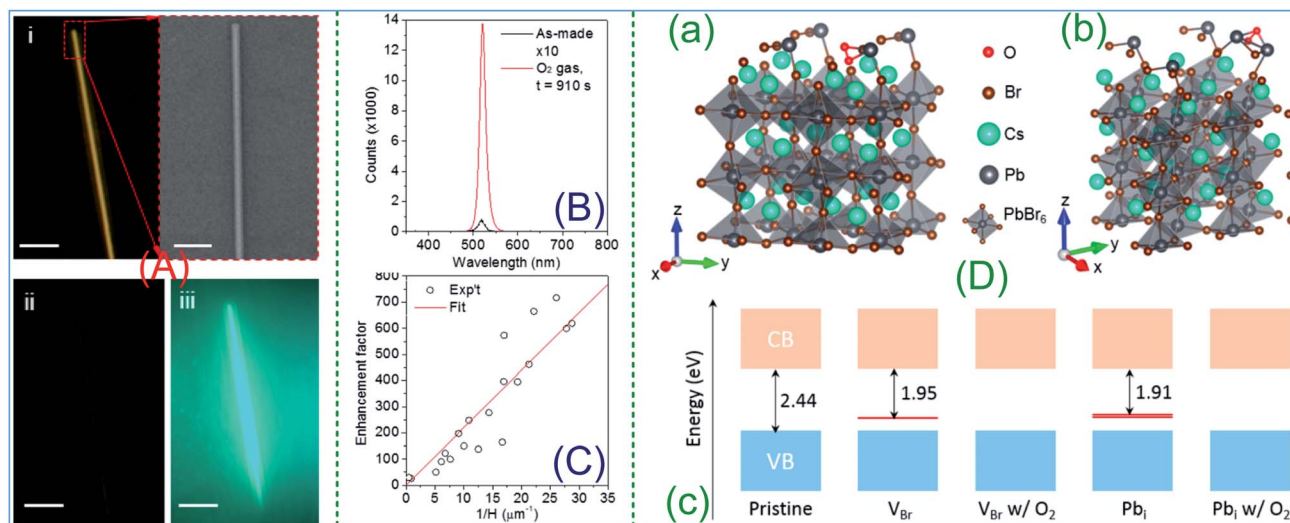
Fig. 15 (A) Optical dark-field image of a CsPbBr 3 NW (i), scale bar, 10 \mu m) with a zoom-in SEM image (scale bar, 1 \mu m). Corresponding PL images for the NW before and after O 2 exposure are shown in (ii) and (iii), respectively (scale bar, 10 \mu m). (B) PL spectra for the as-made CsPbBr 3 NW (black line) and that after O 2 exposure for 910 s (red line). (C) PL enhancement factor plotted against 1/H for individual NWs with sizes varying from \sim 30 nm to a few microns (open circles). (D) Theoretical modeling and energy level calculation. (a and b) Theoretical models of the perovskite surface as a 2D slab with crystal structures for the V Br (a) and Pb i (b) defects adsorbed by an O 2 molecule. V Br , a bromine atom removed from the surface; Pb i , an extra lead atom added to the surface. (c) Theoretical calculated energy levels around the band gap for various defect structures. Bandgaps are shown as the energy difference between the top of the valence band and the bottom of the conduction band. The V Br and Pb i defects introduce occupied deep levels inside the band gap (red lines). In the case of Pb i the defect levels are doubly degenerate. When O 2 is adsorbed onto the defect, the defect levels are removed. Reprinted with permission from ref. 56. Copyright 2018 American Chemical Society.
