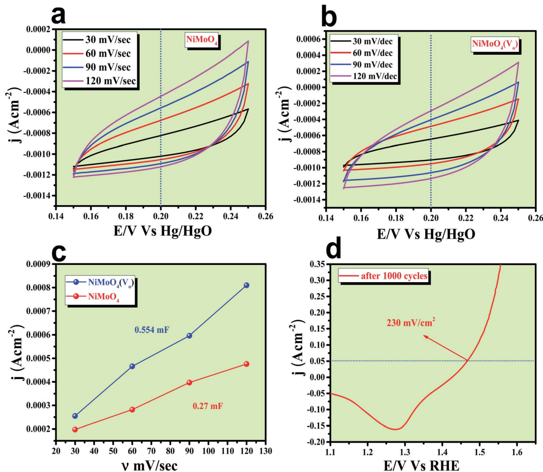
Fig. 8 (a) and (b) Are the CVs recorded for \text{NiMoO}_4 and \text{NiMoO}_4(\text{V}_\circ) respectively in a non-faradaic region with increasing scan rate for the determination of ECSA from its double layer capacitance; (c) are the corresponding plots to the measure C_{dl} ; (d) backward CV after 1000 cycles of AD study.
