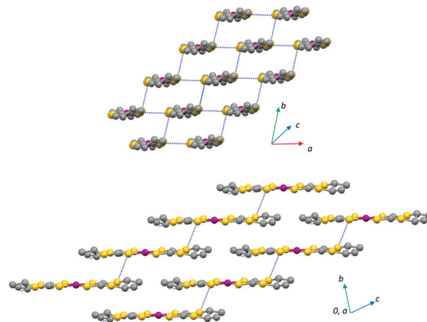
Fig. 16 Detail emphasizing the step-chains like in the crystal structure of [Au(R,R-dm-dddt) 2 ], with blue lines representing S...S short contacts.
