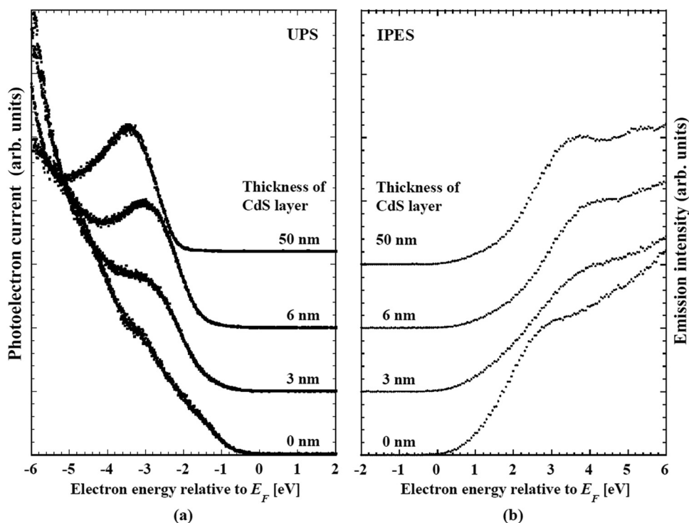
Fig. 20 (a) Changes in the ultraviolet photoemission (UPS) spectra and (b) inverse photoemission (IPES) of CdS-buffer/CIGS Se -absorber structures in conjunction with the thickness of the CdS layer. In both figures, the bottom spectrum indexed with "0 nm" shows nature of the front-surface of the CIGS Se layer.
