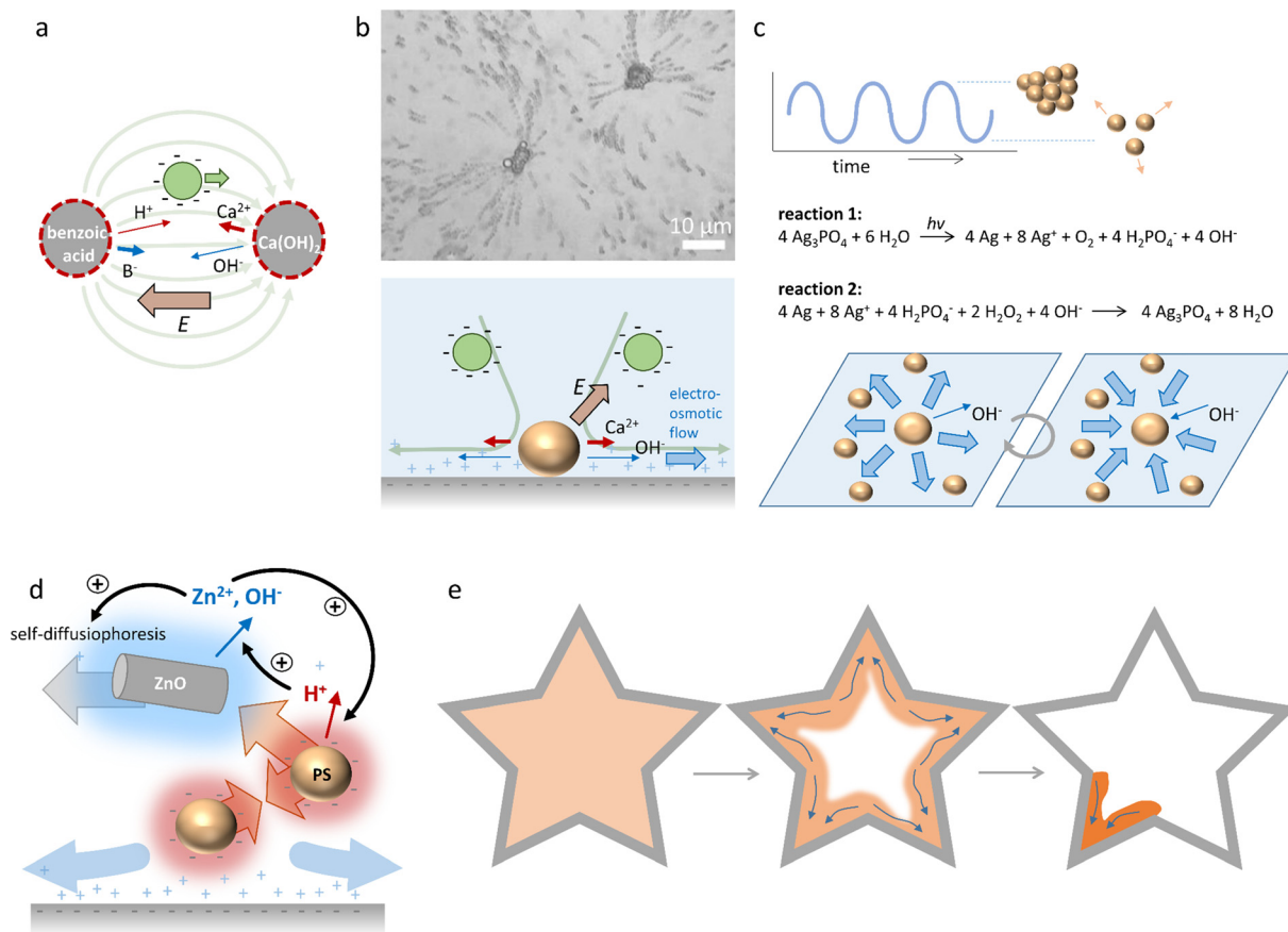
Fig. 15 Self-organisation driven by diffusiophoresis. (a) Motion pattern of negatively charged tracer particles along a sustained pH gradient between benzoic acid and \text{Ca}(\text{OH})_2 sources. 162 (b) Electroosmotic flow drives the motion of tracer particles amongst \text{CaCO}_3 microparticles on a negatively charged substrate. Reprinted (adapted) with permission from ref. 163. Copyright 2012 American Chemical Society. (c) Oscillatory clustering and dispersion of \text{Ag}_3\text{PO}_4 microparticles in an aqueous \text{H}_2\text{O}_2 solution, where reaction (1) and (2) alternate and drive the electroosmotic flow. 170 (d) Diffusiophoretic colloidal swarms based on ZnO nanorods and sulfonated polystyrene microbeads, that are coupled via an ion exchange reaction that provide positive and negative feedback to ZnO/polystyrene clustering. (e) Collective swarm behaviour of ZnO/polystyrene particles (orange) that accumulate in the edge of the geometry (grey) with the highest curvature. 171
