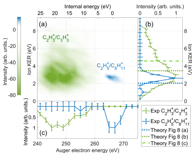
Fig. 9 The difference in energy-resolved AEPIPO data for the C_2H_3^+/C_3H_3^+ (green) and the C_2H_5^+/C_8H_{11}^+ (blue) ion pairs. (a) 2D map showing the energy correlation of the Auger electron energy with the total ion kinetic energy released (KER) for the selected ion pairs. The intensities of the C_2H_3^+/C_3H_3^+ events is set to be negative and the C_2H_5^+/C_8H_{11}^+ events is set to be positive for better contrast in the map. (b) The projection of (a) showing the experimental total ion KER of the C_2H_3^+/C_3H_3^+ (green) and the C_2H_5^+/C_8H_{11}^+ (blue) ion pairs. The theoretical ion KER values obtained from PES (Fig. 8) are shown as vertical dashed lines. (c) The projection of (a) showing the experimental Auger electron energy for the C_2H_3^+/C_3H_3^+ (green) and the C_2H_5^+/C_8H_{11}^+ (blue) ion pairs.
