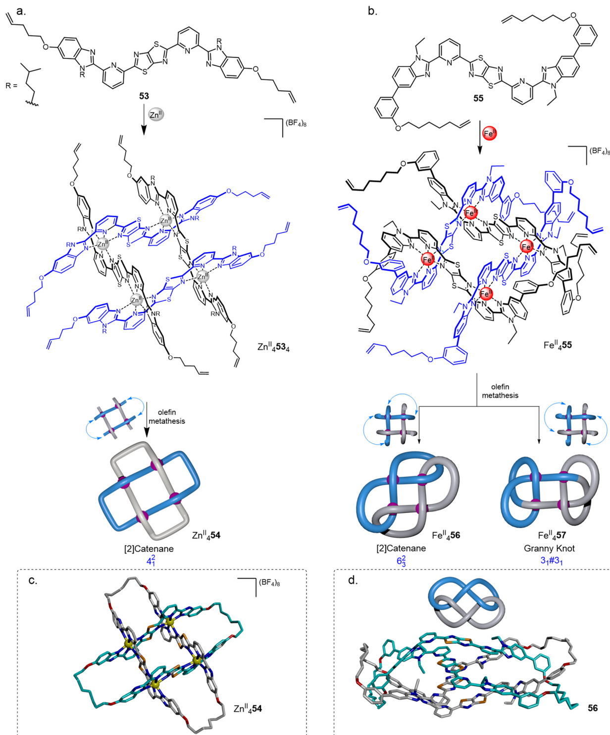
Fig. 20 Synthesis of 2 × 2 interwoven molecular grids and their closures by olefin metathesis to generate (a) Solomon link 54 , 14 or (b) 6^{\text{II}} link 56 and granny knot 57 , 15 X-ray crystal structures of (c) \text{Zn}^{\text{II}} 54 and (d) demetallated link 56 .
