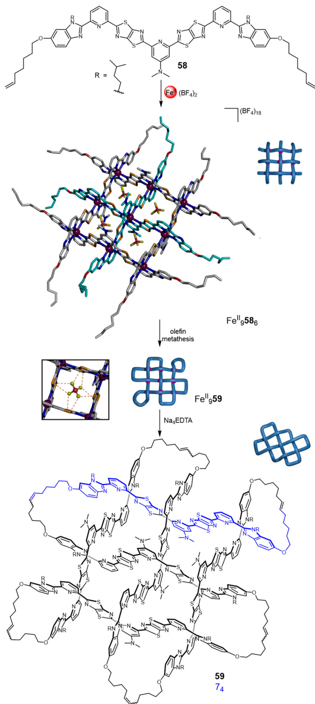
Fig. 21 Weaving molecular endless ( 7_4 ) knot 59 by self-assembly of an interwoven 3 \times 3 grid. 16 Inset: The stabilising effect of the \text{BF}_4^- anions through \text{B}\cdots\text{F}\cdots\pi and electrostatic interactions.
