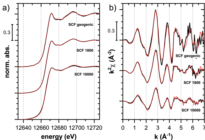
Fig. 8 Tl L_{\text{III}} -edge (a) XANES and (b) EXAFS spectra of a soil clay fraction (SCF) with \sim 260 \text{ mg kg}^{-1} geogenic Tl (SCF geogenic) and with an additional 1800 \text{mg kg}^{-1} (SCF 1800) or 10 000 \text{mg kg}^{-1} freshly adsorbed Tl (SCF 10000) (black lines) and linear fit reconstructions (red lines). LCF results are listed in Table 2.
