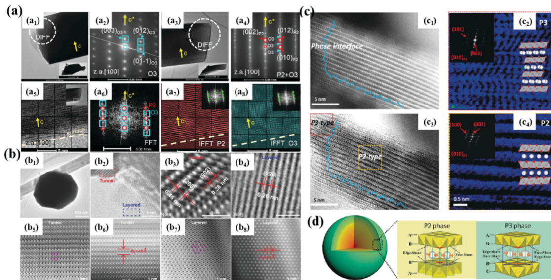
Fig. 7 (a) TEM, SAED, FFT and IFFT patterns of P2/O3 biphase \text{Na}_{0.8}\text{Li}_{0.2}\text{Fe}_{0.2}\text{Mn}_{0.6}\text{O}_2 ; adapted with permission. 31 Copyright 2020, Wiley-VCH. (b) TEM, HR-TEM, HAADF-STEM and ABF-STEM images of layer/tunnel structure materials; 104 (c) HAADF and ABF images of P2@P3NCZM composite material; adapted with permission. 103 Copyright 2018, Wiley-VCH. (d) 3D structural model of the NCZM samples composed of P3 and P2 with the corresponding Na-ion migration paths in different layered structures. Adapted with permission. 105 Copyright 2019, Wiley-VCH.
