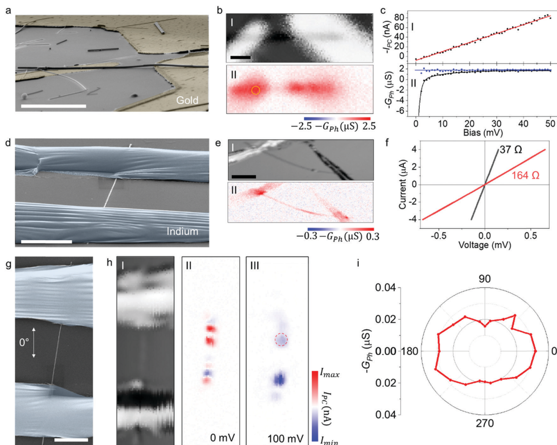
Fig. 3 (a). False colored SEM image of a Ag NW on pre-patterned gold electrodes. Scale bar is 5 \mu\text{m} . (b) Reflection map (I) and the corresponding -G_{\text{ph}} map under 20 mV bias (II) showing the photoconductance over the device. It is noteworthy that there is a significant conductance modulation over the gold electrodes. A 532 nm laser source was used at 65 \mu\text{W} power. The yellow circle indicates the position where -I_{\text{PC}} vs. bias measurements were taken from. The scale bar is 5 \mu\text{m} . (c) -I_{\text{PC}} vs. bias (I) graph showing a linearly increasing -I_{\text{PC}} with the bias (black dots). The red line is the linear fit to the data. Zero bias response is \sim 6 nA. Lower panel (II) shows -G_{\text{ph}} (black dots) and -\frac{I_{\text{PC}} - I_{\text{PC}}^0}{V} (blue dots) vs. bias. Solid lines are fits to the data. (d) False colored SEM image of an indium contacted Ag NW. Note the grating-like structures over the indium, which naturally occur due to thermal contraction upon cooling. Scale bar is 5 \mu\text{m} . (e) Reflection map (I) and the corresponding -G_{\text{ph}} map under 100 mV bias (II) showing the conductance modulation over the indium contacts. Notice that the modulation intensifies near the indium-NW junction. Also, the visible defect in the reflection map results in enhanced plasmonic response, which is clear in the photoconductance map. Data were collected with a 532 nm laser at 96 \mu\text{W} . Scale bar is 10 \mu\text{m} . (f) Current vs. voltage graphs of the same devices, before (red dots) and after (black dots) reduction of the photoconductance. (g) False colored SEM image of a device with the incident polarization angle marked. (h) (I) Reflection map, (II) open-circuit response, and (III) 100 mV response maps are shown. I_{\text{max}} = 0.25 nA for (II), 25 nA for (III) and I_{\text{min}} = -0.25 nA for (II) and -25 nA for (III). (i) The polar chart shows the incident polarization angle vs. -G_{\text{ph}} at 100 mV bias. The data were collected from the individual maps taken around the red dashed circle in h (III).
