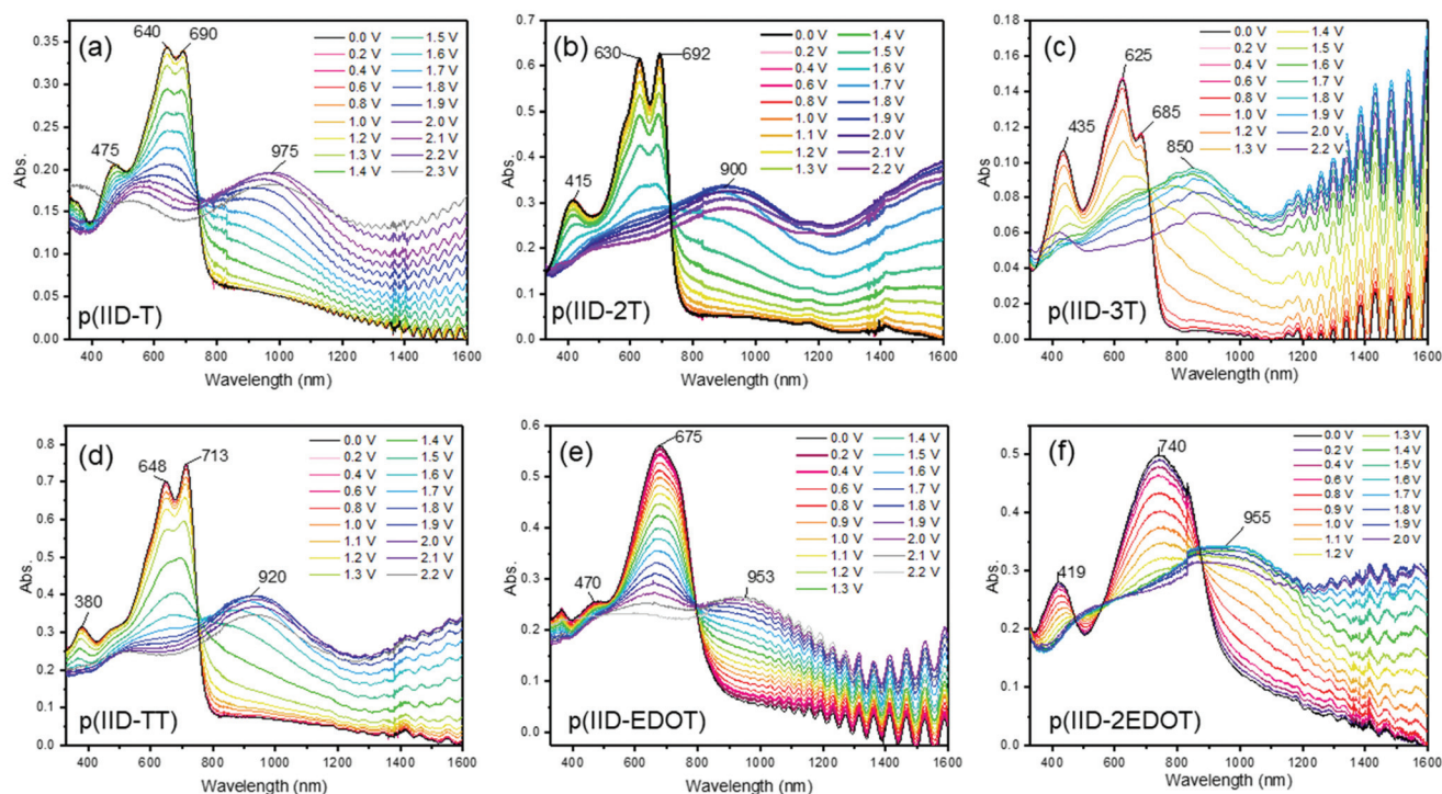
Fig. 1 Spectroelectrochemistry of isoidingo polymers (a) p(IID-T) , (b) p(IID-2T) , (c) p(IID-3T) , (d) p(IID-TT) , (e) p(IID-EDOT) and (f) p(IID-2EDOT) in fabricated ECDs, undergoing electrochemical oxidative doping.
