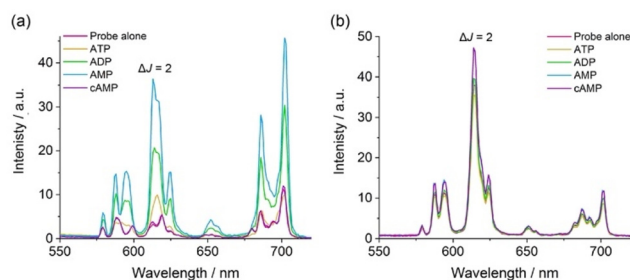
Fig. 4 (a) Large enhancement in emission intensity of [\text{Eu}\text{-pBOH}_2]^+ with AMP (1 mM) compared with ATP, ADP and cAMP (1 mM each). (b) Lack of response of [\text{Eu}\text{-oBOH}_2]^+ towards nucleoside phosphate anions. All spectra measured using 5 \mu\text{M} \text{Eu}(\text{III}) complex in 10 mM HEPES at pH 7.0 and 295 K, \lambda_{\text{exc}} = 322 \text{ nm} .
