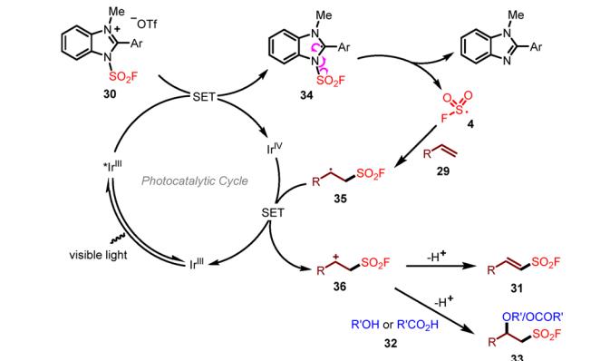
Scheme 5 Photoredox-catalyzed radical fluorosulfonylation of alkenes with a benzoimidazolium-based fluorosulfonyl radical precursor.
