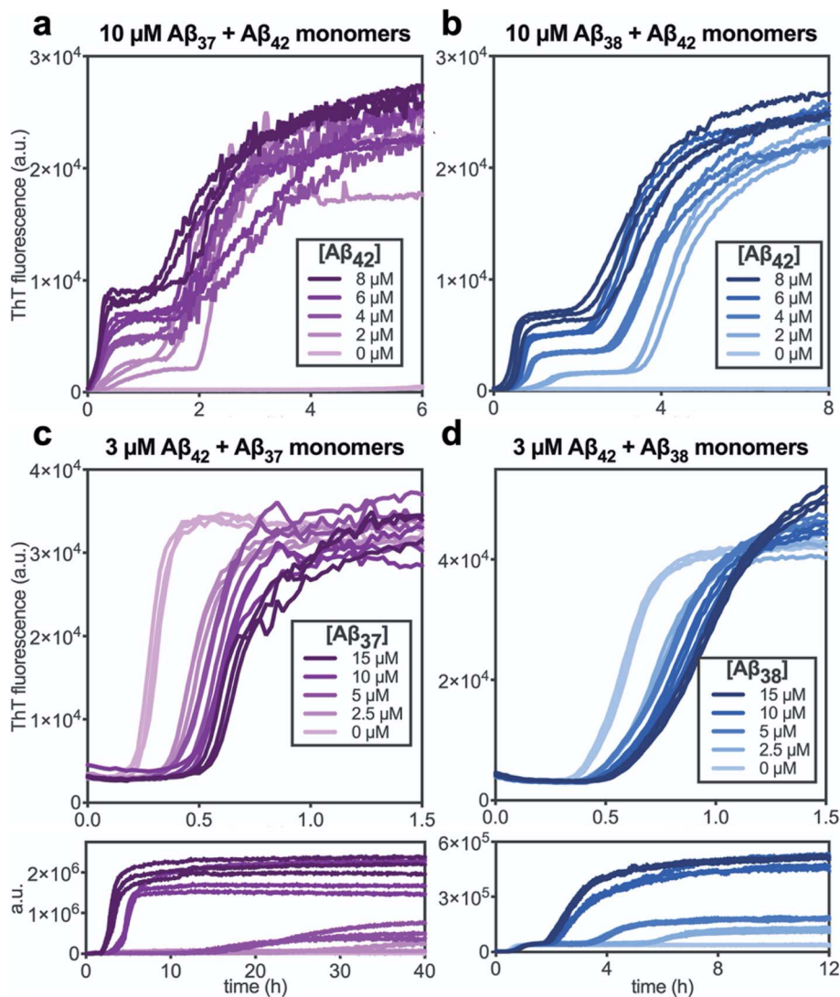
Fig. 6 Aggregation kinetics of two-peptide systems composed of A\beta_{42} with (a & c) A\beta_{37} and (b & d) A\beta_{38} in 20 mM sodium phosphate buffer, pH 7.4, with 200 \mu M EDTA, 0.02% Na_3N , and 20 \mu M ThT. (a and b) Increasing A\beta_{42} concentration leads to accelerated aggregation of A\beta_{37} and A\beta_{38} , respectively. Aggregation kinetics for A\beta_{42} alone at the same concentrations are shown in Fig. S1.† (c and d) Increasing concentrations of A\beta_{37} and A\beta_{38} , respectively, decrease the rate of A\beta_{42} aggregation; in both, the upper panel shows the first, low-intensity fluorescence transition and the lower panel shows the full biphasic aggregation profile.
