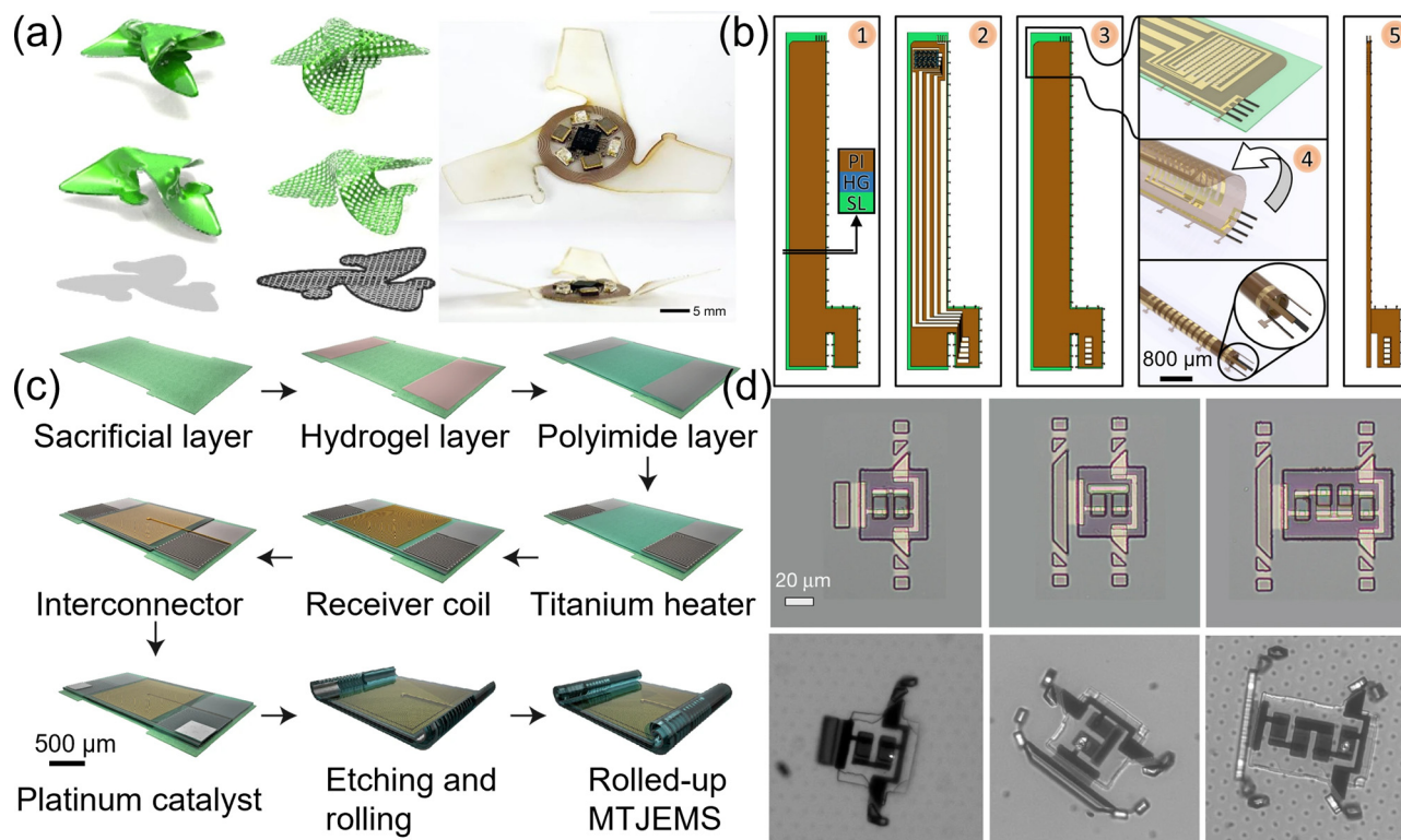
Fig. 2 Semiconductor and microelectronic techniques. (a) Seed-inspired 3D electronic microfliers. Scale bar, 5 mm. Reproduced with permission 2 . Copyright 2021, Springer Nature. (b) Integrated self-assembled catheter with electronic components. Reproduced with permission. 109 Scale bar, 800 μm. Copyright 2021, American Association for the Advancement of Science. (c) Fabrication schematics of a motile twin-jet-engine microsystem. Scale bar, 500 μm. Reproduced with permission. 72 Copyright 2020, Springer Nature. (d) Microscopic robot with internal electronics fabricated by semiconductor techniques. Scale bar, 20 μm. Reproduced with permission. 39 Copyright 2020, Springer Nature.
