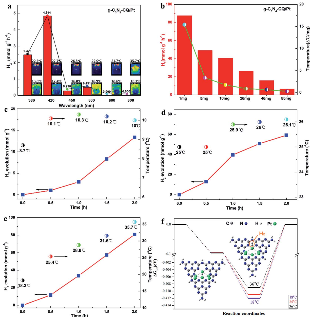
Fig. 1 STAP \text{H}_2 evolution. (a) Relationships between the PHE rate and heating effects of typical monochromatic light in the solar spectrum. Photocatalyst loading: 10 mg. (b) Dependence of the PHE rate and system temperature elevation on the photocatalyst loading. (c) PHE rate for the system temperature controlled at 10^{\circ}\text{C} \pm 1^{\circ}\text{C} . (d) PHE rate for the system temperature controlled at 25^{\circ}\text{C} \pm 1^{\circ}\text{C} . (e) PHE rate for the solar thermal system with variable increasing temperatures. (f) Calculated Gibbs energy ( \Delta G_{\text{A}} ) of H-atom adsorption and Gibbs energy ( \Delta G_{\text{D}} ) of \text{H}_2 molecule desorption. Inset: structural model for the H atom and \text{H}_2 molecule adsorbed on Pt sites.
