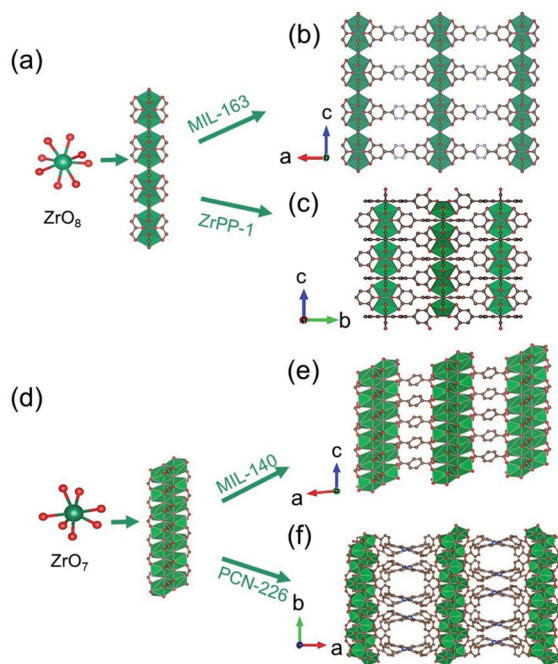
Fig. 16 (a) The infinite 1D Zr^{(iv)} -oxo chain assembled from ZrO_8 polyhedrons; (b) corresponding framework structure of MIL-163. Reproduced with permission from ref. 106. Copyright 2015, WILEY-VCH Verlag GmbH. (c) The corresponding framework structure of ZrPP-1. Reproduced with permission from ref. 34. Copyright 2018, WILEY-VCH Verlag GmbH. (d) The infinite zigzag 1D Zr^{(iv)} -oxo chain assembled from ZrO_7 polyhedrons; (e) corresponding framework structure of MIL-140. Reproduced with permission from ref. 30. Copyright 2021, WILEY-VCH Verlag GmbH. (f) The corresponding framework structure of PCN-226. Reproduced with permission from ref. 32. Copyright 2020, American Chemical Society.
