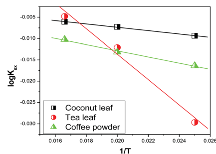
Fig. 7 The variation in equilibrium sorption constants as a function of the reciprocal of the temperature ( 1/T , K); sorbent amount: 20 mg, aqueous phase volume: 1.5 mL, initial Th concentration: 2 mg mL -1 , equilibration time: 4 h, centrifugation time: 2 min, aqueous phase acidity: 3 M HNO 3 .
