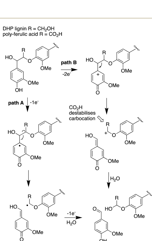
Fig. 7 Mechanisms for α,β-bond cleavage of β-aryl ether lignin units in DHP lignin (R = CH 2 OH) or poly-ferulic acid (R = CO 2 H). Path A, radical mechanism proposed for R. jostii RHA1 peroxidase DypB; 7 path B, possible 2-electron mechanism for oxidative cleavage.
