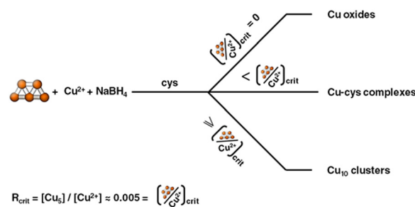
Fig. 4 Scheme representing the products obtained after reaction of \text{CuNO}_3 , cysteine and \text{NaBH}_4 using different amounts of catalytic \text{Cu}_5 clusters.
