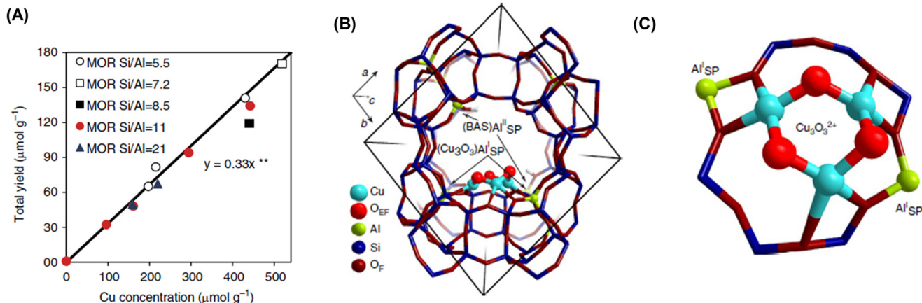
Fig. 9 (A) Total yield of methanol over Cu-MOR with different Si/Al ratios and Cu concentrations. (B) Location and (C) structure of [Cu_3(\mu-O)_3]^{2+} cluster in MOR determined by DFT calculations. Reproduced from ref. 47 with permission from Springer Nature, copyright 2015.
