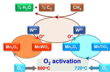
Fig. 6 Proposed catalytic cycle for OCM reaction mediated by the redox cycle \text{Mn}^{2+} \rightarrow \text{Mn}^{3+} over \text{Mn-Na}_2\text{WO}_4/\text{Ti-MWW} . Reprinted from ref. 36 with permission from The American Association for the Advancement of Science, copyright 2017.
