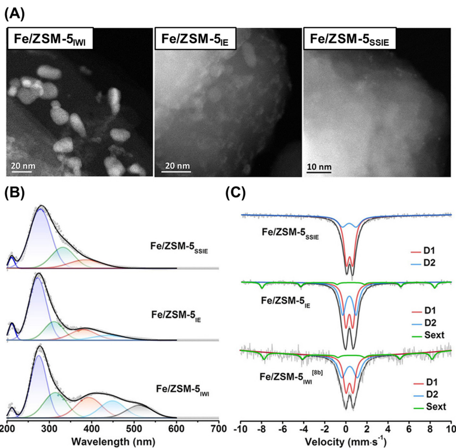
Fig. 15 (A) STEM images, (B) UV-vis spectra, and (C) 57 Fe Mössbauer spectra of Fe/ZSM-5s. Reprinted from ref. 65 with permission from John Wiley and Sons, copyright 2021.
