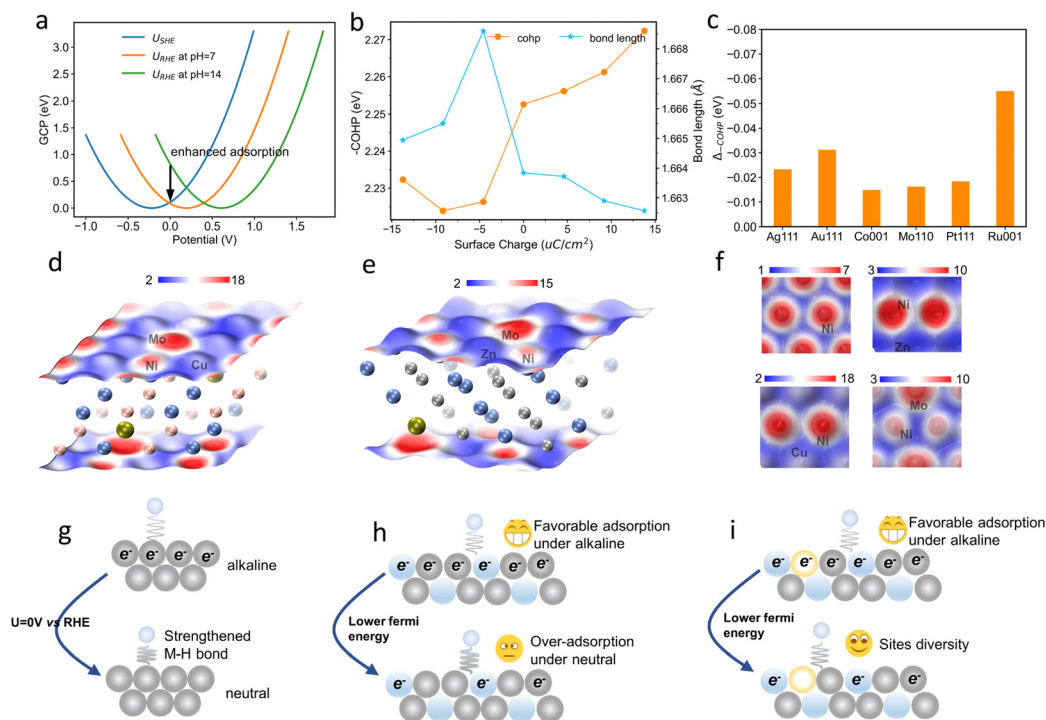
Fig. 7 Surface reactivity diversity and pH-dependent hydrogen adsorption. (a) GCP based hydrogen adsorption free energies. (b) COHP and bond length of the Ni–H bond. (c) ICOHP changes as the surface charge becomes more negative. (d)–(f) Fermi softness of various surfaces. (g) The schematic representation of the surface reactivity diversity enabled pH-universal HER. Ni, Mo, Cu, and H atoms are shown as light-grey, blue-grey, light-yellow, and white balls, respectively.
