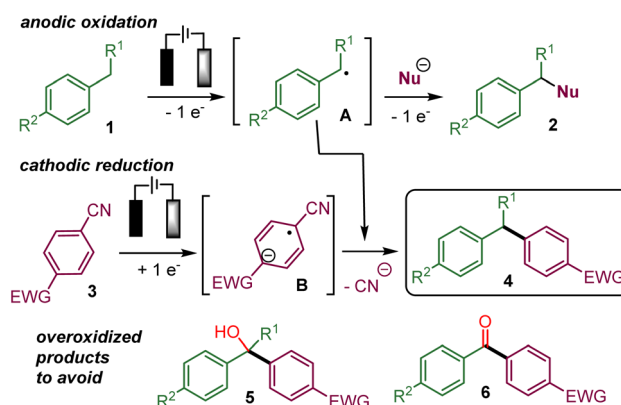
Scheme 1 The proposed electrochemical benzylic arylation via convergent paired electrolysis.
