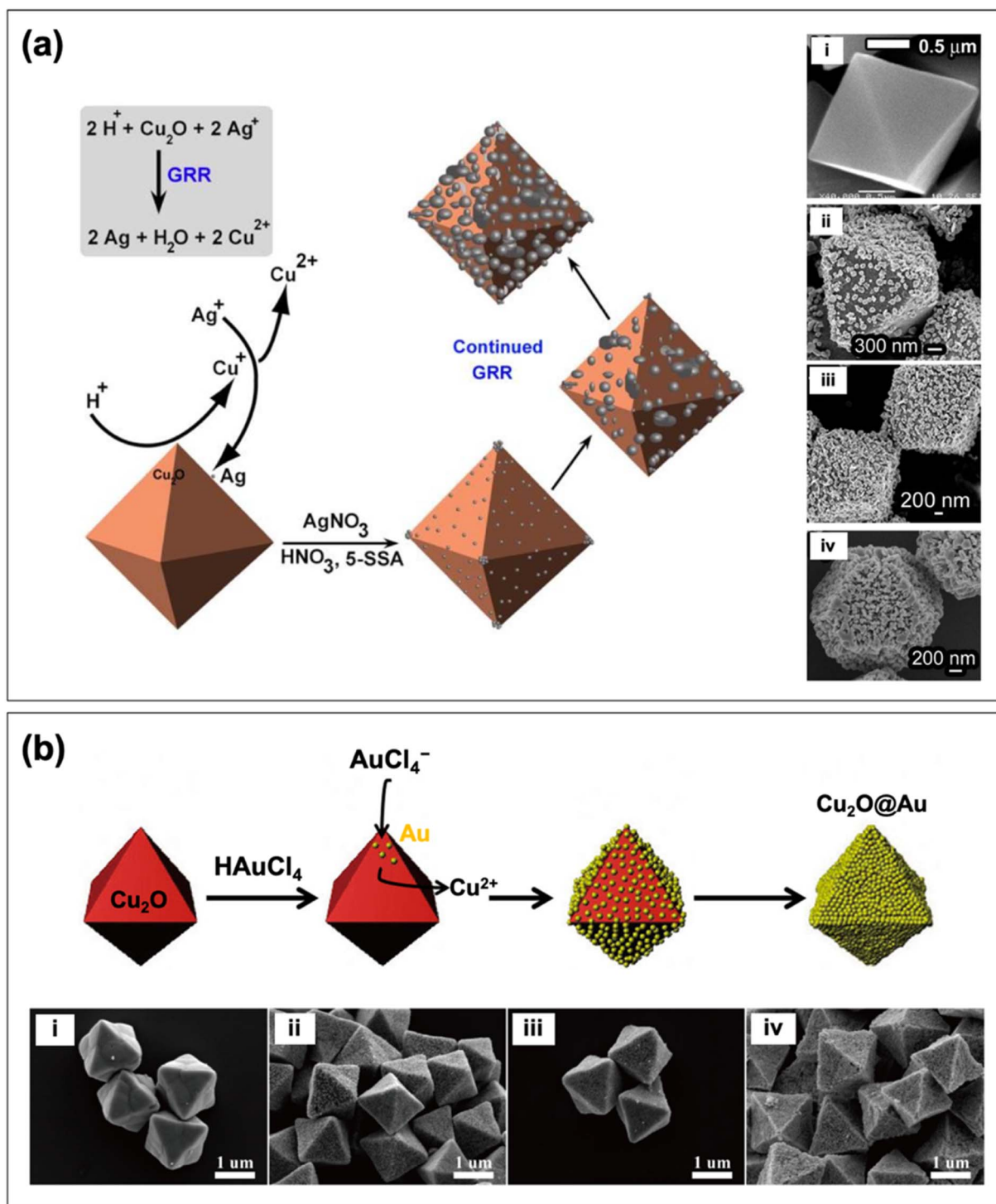
Fig. 4 Schematic depiction of the formation of (a) \text{Cu}_2\text{O}@\text{Ag} and (b) \text{Cu}_2\text{O}@\text{Au} core-shell nanocomposites through GRR. Also shown are the SEM images of the structures produced with (i) no metal and (iii) to (iv) increasing loading amount of metal. Reproduced with permission from (a) ref. 69, copyright 2017 the Royal Society of Chemistry, and (b) ref. 62, copyright 2016 Elsevier.
