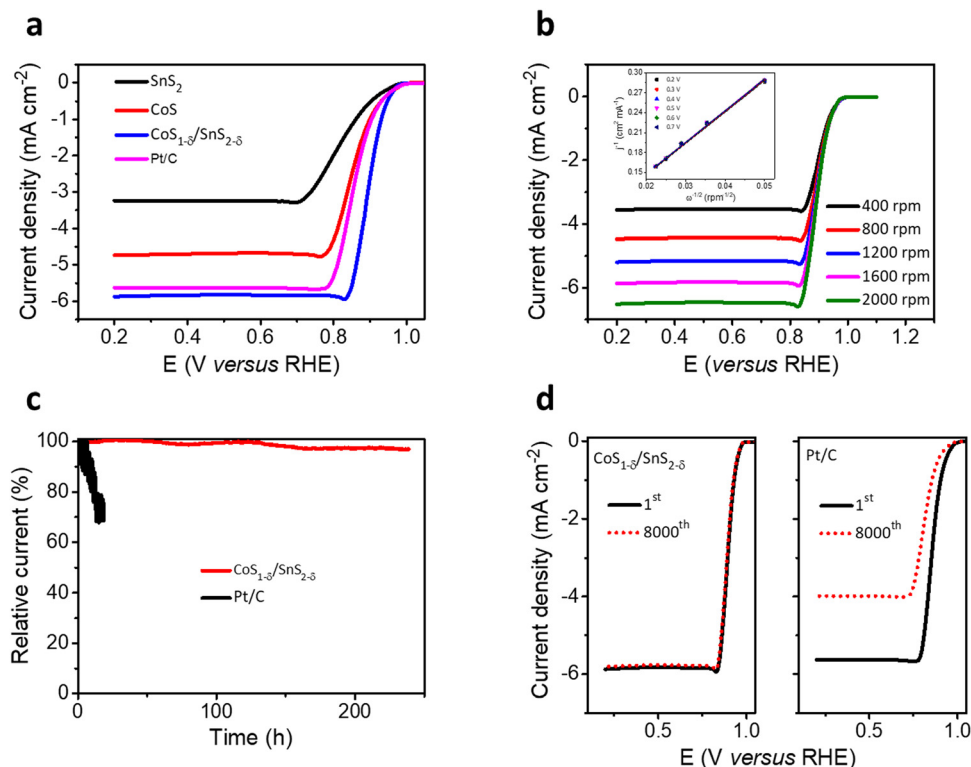
Fig. 3 ORR electrochemical performances. (a) LSV polarizations for the \text{CoS}_{1-\delta}/\text{SnS}_{2-\delta} hetero-interface related to those of \text{SnS}_2 , \text{CoS} , and reference Pt/C materials. (b) RDE profiles for \text{CoS}_{1-\delta}/\text{SnS}_{2-\delta} materials. Sweeping rates of 400–2000 rpm. K–L polarizations for electrochemical kinetics with \text{CoS}_{1-\delta}/\text{SnS}_{2-\delta} materials from 0.2 to 0.7 V (inset). (c) Chronoamperometric ( i-t ) tests for \text{CoS}_{1-\delta}/\text{SnS}_{2-\delta} referenced to that of commercial Pt/C at their relevant half-wave potentials. (d) ORR-accelerated operations for \text{CoS}_{1-\delta}/\text{SnS}_{2-\delta} and reference Pt/C materials for the initial cycle and after 8000 cycles. (Conditions: 0.1 M KOH and geometrical surface area utilized for current density calibration.)
