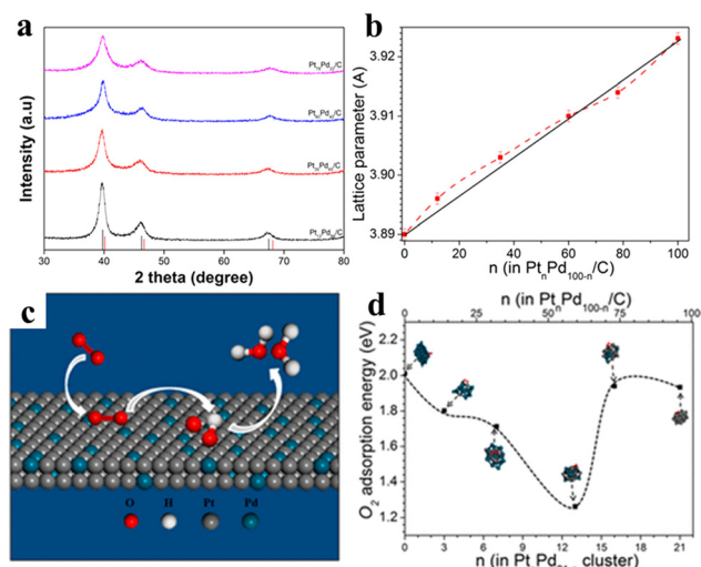
Fig. 27 (a) XRD patterns of Pt 12 Pd 88 /C, Pt 35 Pd 65 /C, Pt 60 Pd 40 /C, and Pt 78 Pd 22 /C nanowires (b) lattice parameters for PtnPd 100-n NWs/C on the relative composition of Pt%, the solid black line is according to Vegard's law based on the lattice parameters of Pt and Pd. (c) Schematic illustration of the catalytic synergy for the ORR over PtPd nanowires featuring the (111) facet. (d) Adsorption energy for molecularly adsorbed O on PtnPd 21-n clusters ( n = 1-21 ) obtained by DFT calculations. Reprinted with permission from ref. 112. Copyright 2020 from the American Chemical Society.
