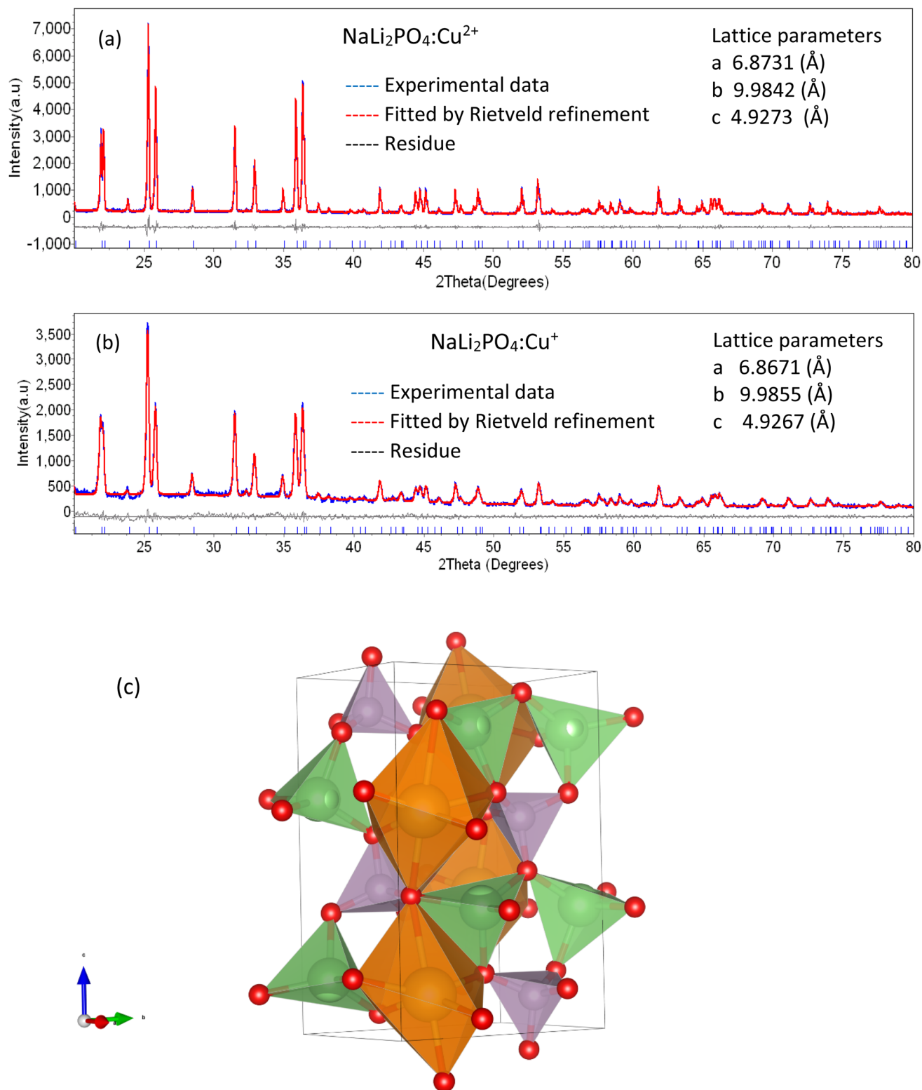
Fig. 1 PXRD patterns of the NaLi 2 PO 4 phosphors: (a) PXRD pattern of the NaLi 2 PO 4 :Cu(II) phosphor material, (b) PXRD pattern of the NaLi 2 PO 4 :Cu(I) phosphor material, (c) crystal structure. Theoretically fitted by Rietveld refinement patterns along with JCPDS data (file # 80-2110) are shown for comparison. The lattice parameters used for the fittings are also shown in the inset.
