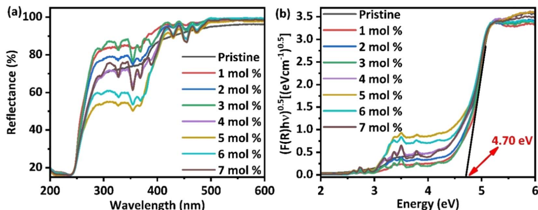
Fig. 2 (a) Diffusive reflectance spectra for \text{Ba}(\text{La}_{2-x}\text{Dy}_x)\text{ZnO}_5 ( x = 0\text{--}7 mol%) phosphor (b) Tauc's plot for estimating the indirect bandgap of synthesized phosphor materials.
