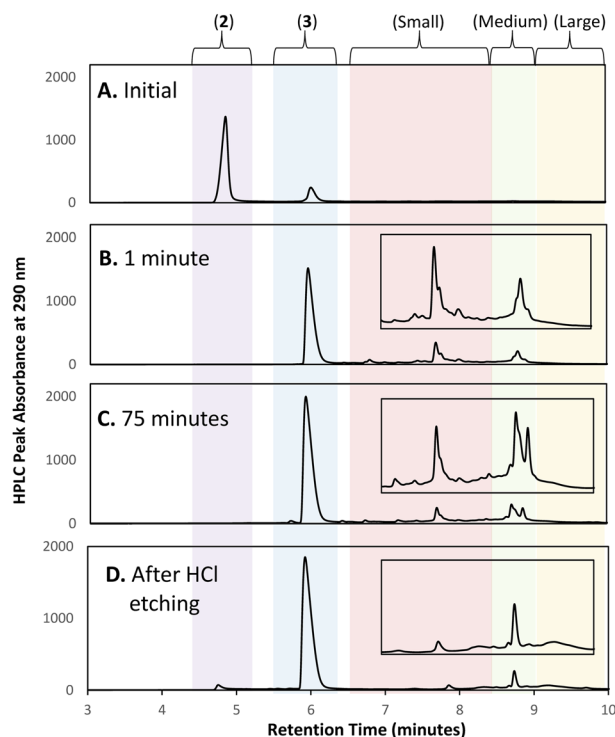
Fig. 2 Chromatograms of the synthesis of 4 taken at four critical points in the reaction with regional analysis zones identified and highlighted. Sample taken before the addition of \text{NaBH}_4 (A), immediately following addition of \text{NaBH}_4 (B), after 75 minutes of reaction time (C), and after HCl etching (D).
