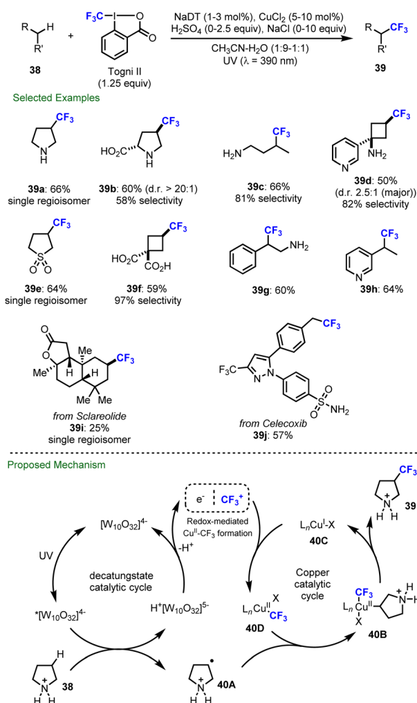
Scheme 10 Direct \text{C}(\text{sp}^3)\text{--H} trifluoromethylation via decatungstate and copper catalysis.
