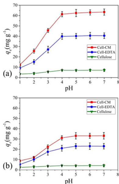
Fig. 15 Adsorption efficiencies of extracted cellulose, cell-EDTA (ethylene diamine tetra acetic acid-modified nanocellulose), and cell-CM (carboxy methyl group-modified nanocellulose) for (a) Pb^{2+} and (b) Cd^{2+} in the pH range of 1–7. Conditions for adsorption: concentration of Pb^{2+} or Cd^{2+} = 100\text{ mg L}^{-1} , at room temperature for 90 min. 81
