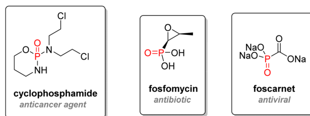
Fig. 14 Early organophosphorus therapeutics.
