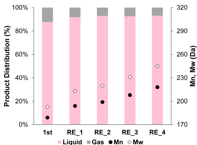
Fig. 12 Product distribution (liquid and gas) and M_n and M_w from OL after the first hydrogenolysis and 4 consecutive recycling experiments using 2cPt cal+red /STO. Conditions: i -PP (3 g), 301.0 mg 2cPt cal+red /STO catalyst, 300 °C, 180 psi mixed gas, 24 h. For gas distribution, see ESI. † No solid products were observed. D = 1.1 for all.
