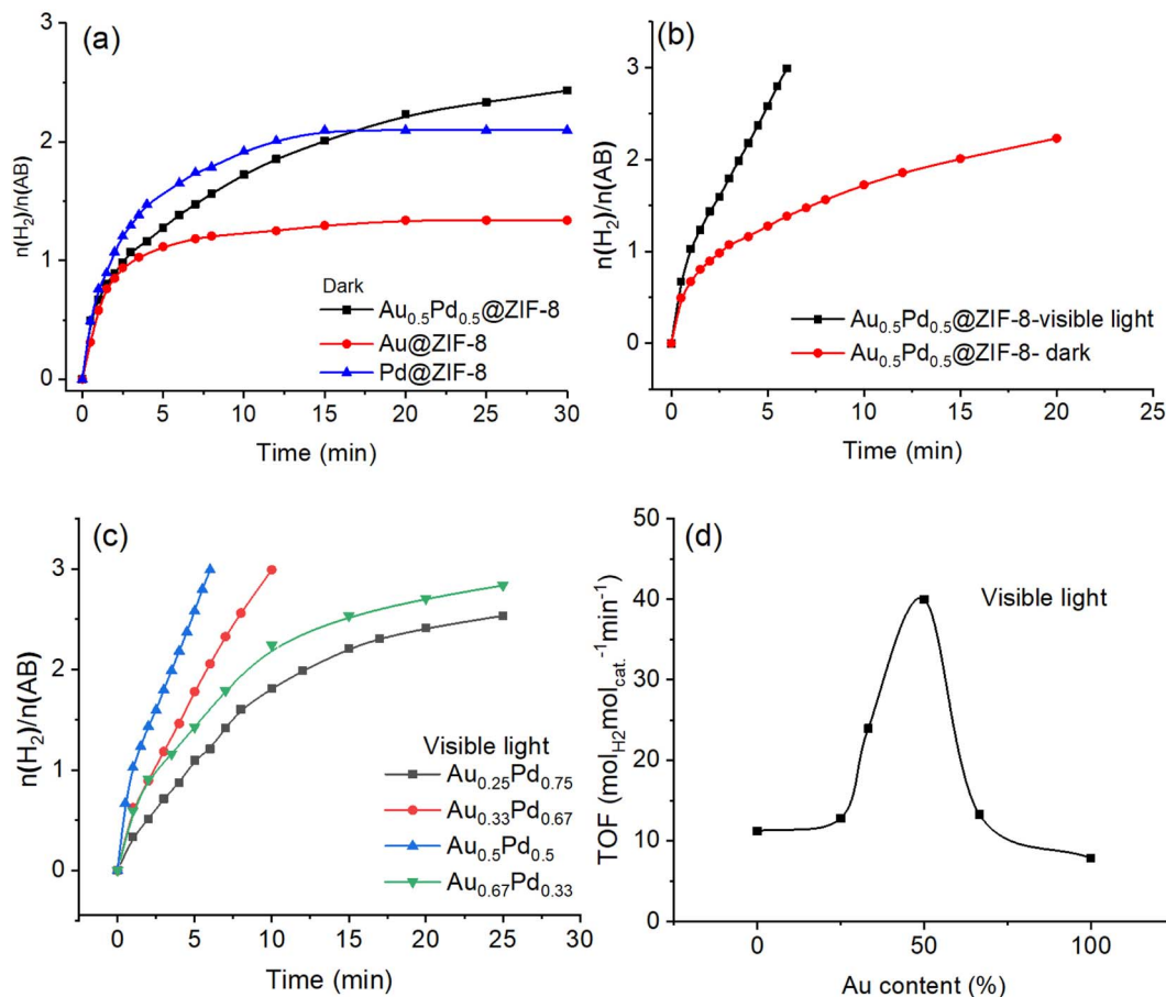
Fig. 2 (a) Plot of the amount of mol \text{H}_2 released during AB methanolytic dehydrogenation vs. time catalyzed by \text{AuNP}@ZIF-8 , \text{PdNP}@ZIF-8 and \text{Au}_{0.5}\text{Pd}_{0.5}\text{NP}@ZIF-8 . (b) Compared efficiencies of the nanocatalysts among \text{Au}_{0.5}\text{Pd}_{0.5}@ZIF-8 without illumination by visible light. (c) Plot of the amount of mol \text{H}_2 released upon methanolytic dehydrogenation of AB vs. time catalyzed by \text{Au}_{0.5}\text{Pd}_{0.5}@ZIF-8 with different ratios of Au and Pd with illumination using visible light. (d) Values of TOFs with various ratios of Au/Pd upon illumination with visible light. In all experiments, the conditions are as follows: 1 mmol of AB; 1.25% mmol MNP; and temperature: 25 \pm 0.5 °C.
