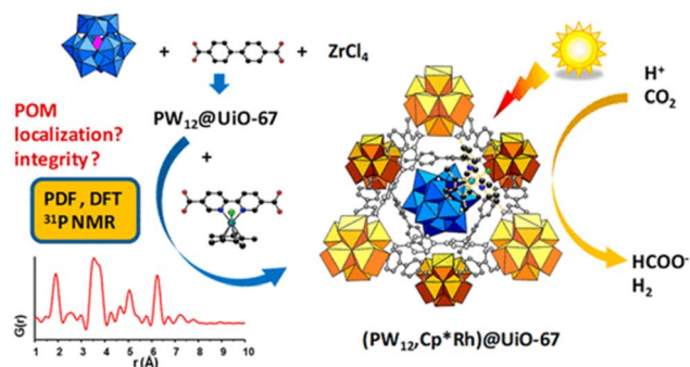
Scheme 8 Scheme for photocatalytic reduction of \text{CO}_2 to produce formate catalyzed by (\text{PW}_{12}\text{Cp}^*\text{Rh}) @UiO-67. Reprinted from ref. 89 with permission from American Chemical Society (Copyright 2020).
