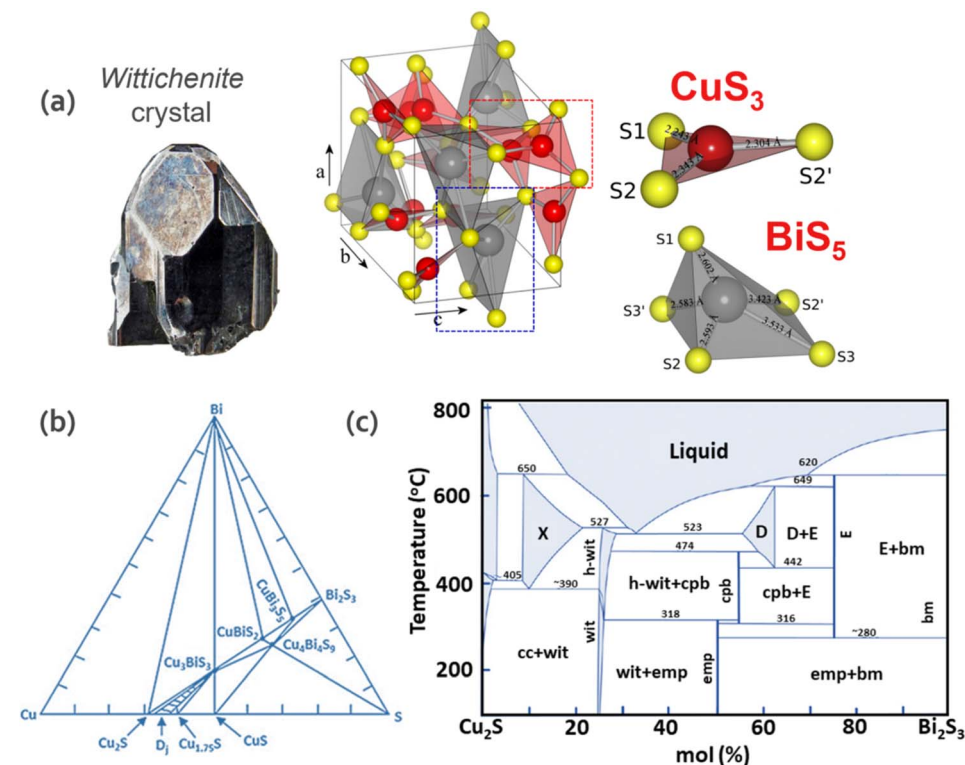
Fig. 2 (a) Orthorhombic crystal structure of wittichenite (CBS), trigonal planar CuS 3 unit showing distances between Cu (red) and S (yellow) atoms and distorted square pyramidal BiS 5 unit showing distances between Bi (grey) and S (yellow) atoms. Adapted with permission from ref. 31 Copyright 2012 Elsevier B.V. (b) Triangle phase diagram of the Cu–Bi–S system at 300 °C. Adapted from the thesis of Chamorro et al. 32 (c) Binary phase diagram of the Cu 2 S–Bi 2 S 3 system. wit = CBS, h-wit = high form CBS, emp = emplectite, cpb = Cu 4 Bi 7 S 12 , X = Cu 9 BiS 6 , D = Cu 3 Bi 5 S 9 , E = CuBi 3 S 5 cc = Cu 2 S, and bm = Bi 2 S 3 . 33
