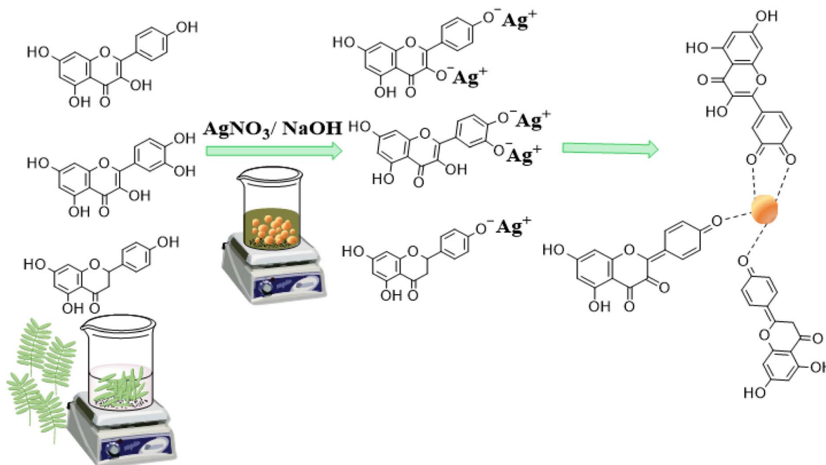
Scheme 1 Illustration of the reaction mechanism for the AgNP synthesis.
