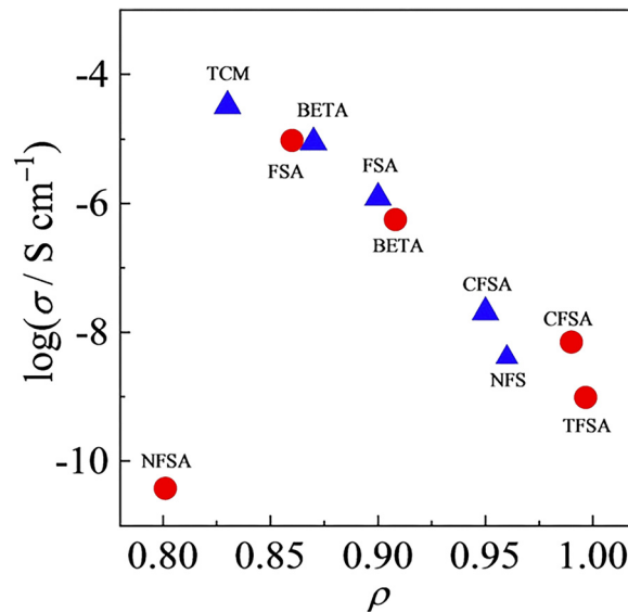
Fig. 4 Relationship between ionic conductivity value at 25 °C and \rho for 1 - (blue triangle) and 3 -based salts with various anion species. Reprinted from ref. 57 with permission.
