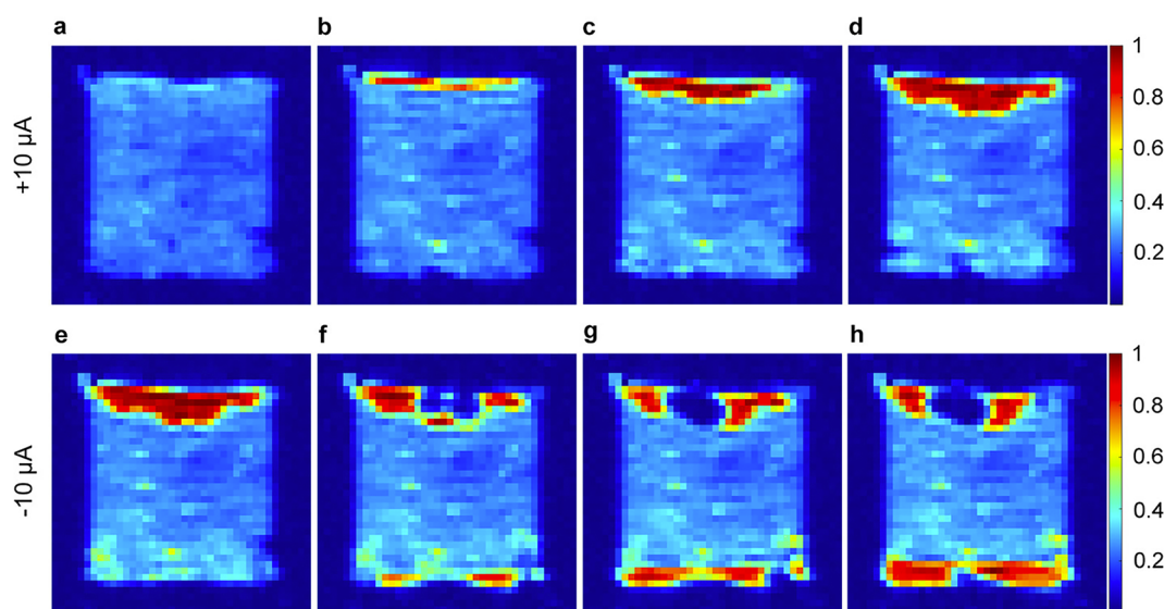
Fig. 6 ^1\text{H} SPRITE images of a symmetric cell (Li coated Cu disks) with 4 mol % LiFSA-doped 28b electrolyte under galvanostatic conditions. (a) Initial cell then continuous application of +10 \mu\text{A} for (b) 17 h, (c) 34 h, and (d) 51 h; and reversed polarity ( -10 \mu\text{A} ) for the same cell for (e) 6 h, (f) 40 h, (g) 57 h, and (h) 77 h. Reprinted from ref. 69 with permission.
